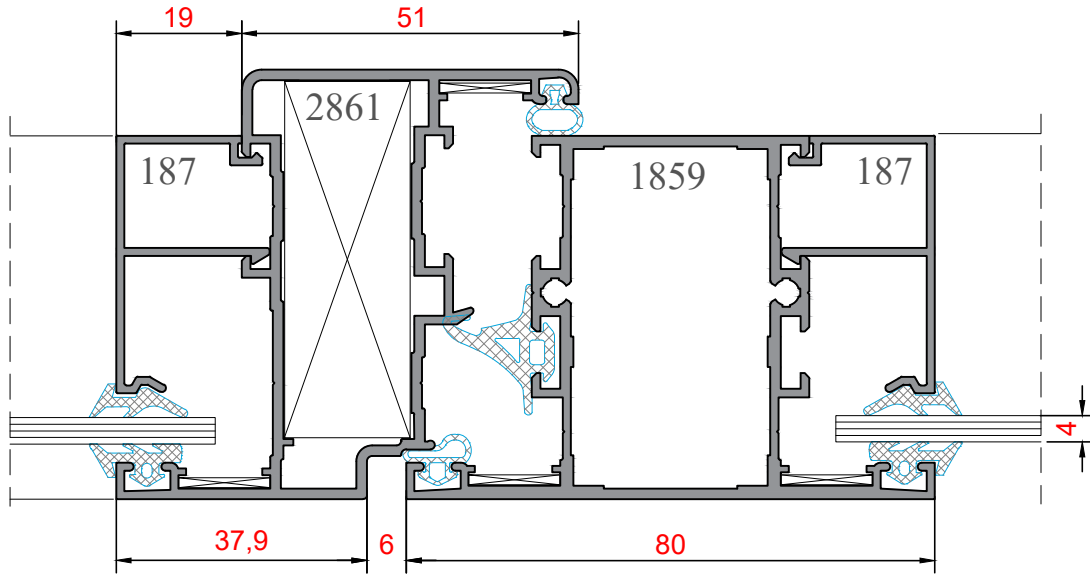
DETAY 2 DETAIL 2
