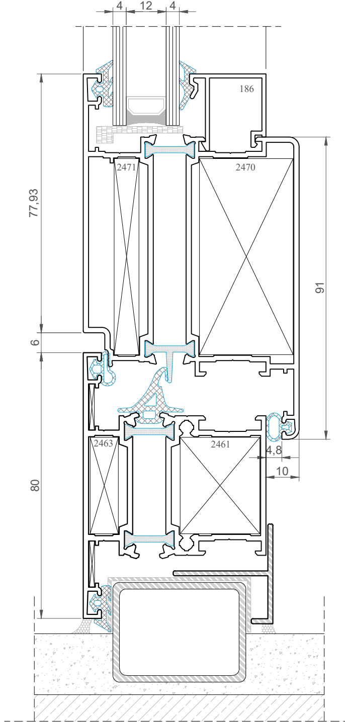
DETAY DETAIL 1
