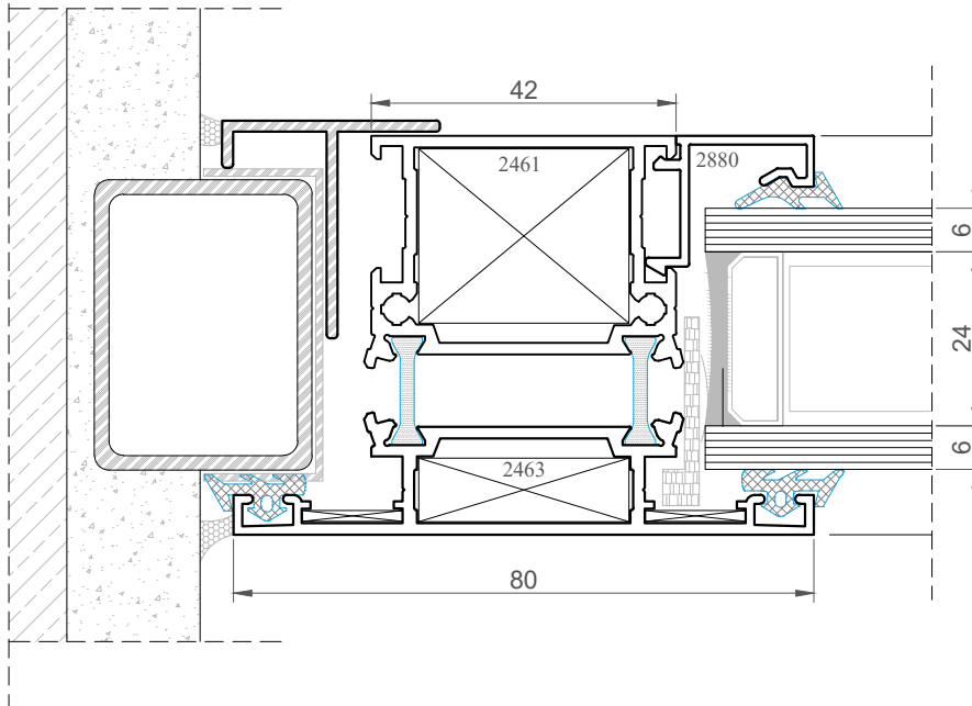
DETAY DETAIL 1
