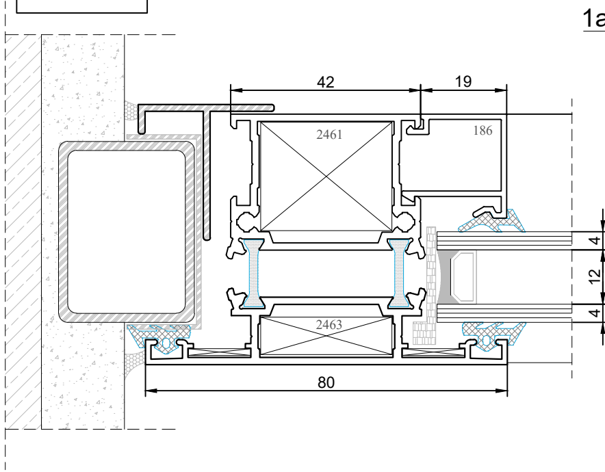
DETAY DETAIL 1
