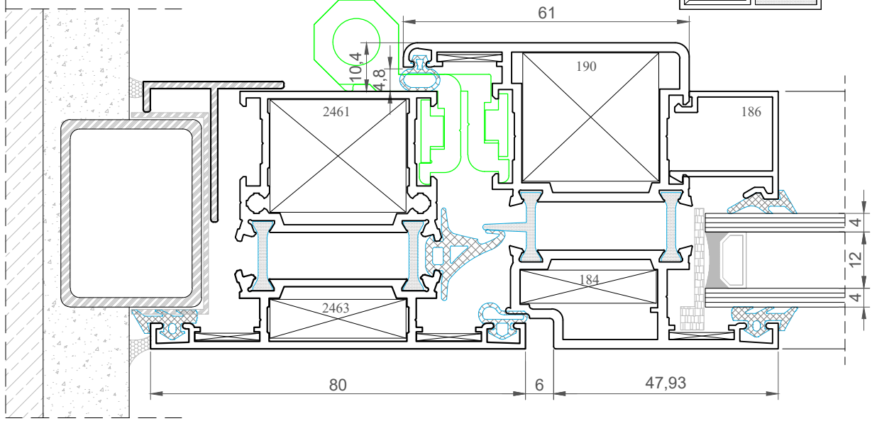
DETAY DETAIL 1
